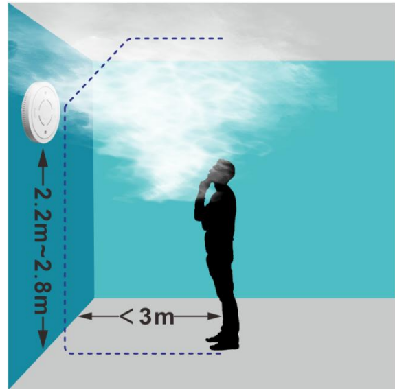
Figure 9–3 Installed on walls
